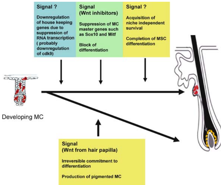
Fig. 3. Three steps during the induction of the quiescent stem cell, which is regulated extrinsically by the microenvironment. During neonatal development, melanocyte differentiation diverges into two pathways. One is to undergo irreversible commitment to mature melanocytes with pigmentation, which takes place in the population migrating to the hair matrix. The second pathway is possible only for the melanocytes remaining in the upper part of the developing hair follicles. From gene expression analysis, three distinct steps are supposed to be required for inducing quiescent stem cells. At the end of these processes, the stem cell acquires a cell-autonomous survival ability
