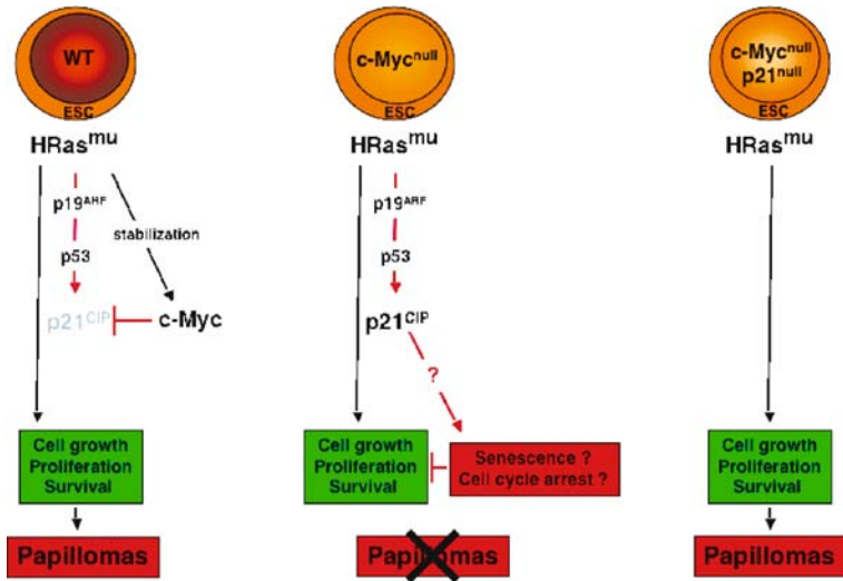
Fig. 1. Model showing the differential response of DMBA/TPA-treated wild-type (WT, left ), c-Myc^{null} ( middle ) and c-Myc^{null} , p21^{null} double mutant ( right ) epidermal stem cells (ESCs) to develop papillomas. In WT mice, activated HRas ( HRas^{mu} ) increases p21^{CIP1} expression but also stabilizes endogenous c-Myc , which in turn represses p21^{CIP1} expression. The pro-oncogenic activities of HRas^{mu} include the promotion of cellular growth, proliferation, and survival, which lead to the formation of papillomas ( left ). In a c-Myc -deficient situation ( middle ), p21^{CIP1} expression is not repressed, causing the activation of a cell cycle arrest and senescence program, which prevents the development of papillomas ( middle ). ESCs lacking both c-Myc and p21^{CIP1} are able to develop papillomas, showing that the single main function of c-Myc during HRas^{mu} -driven papillomagenesis is to repress p21^{CIP1} .
